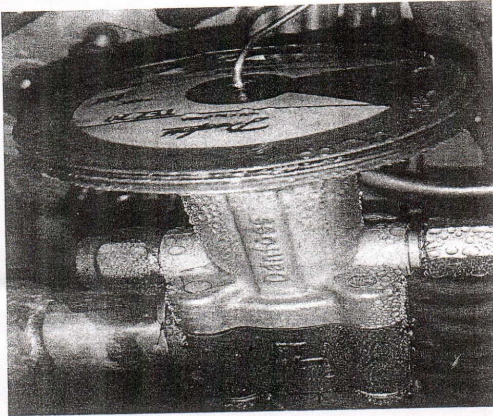
Fig- Expansion Valve
