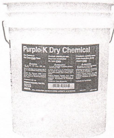
Fig: Chemical, Potassium bicarbonate KHCO 3
