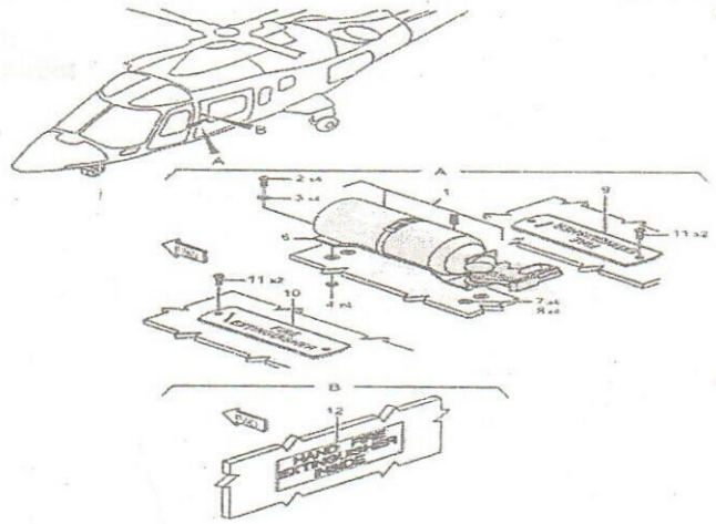
Fig: Fire Extinguisher Assy
