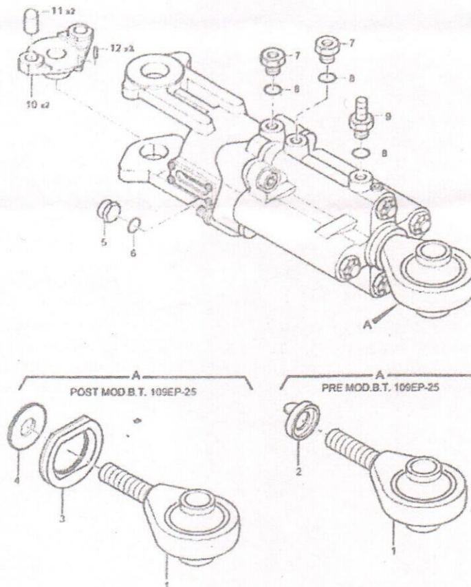
Fig: Damper Assy
