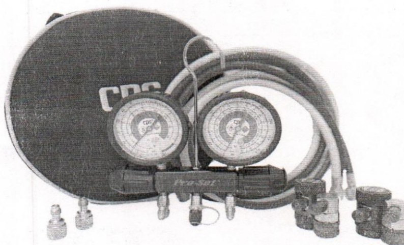
Automotive Manifold Kit
